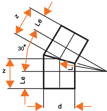
Elbow 30°
