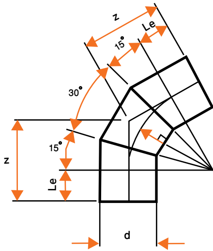
Elbow 60°
